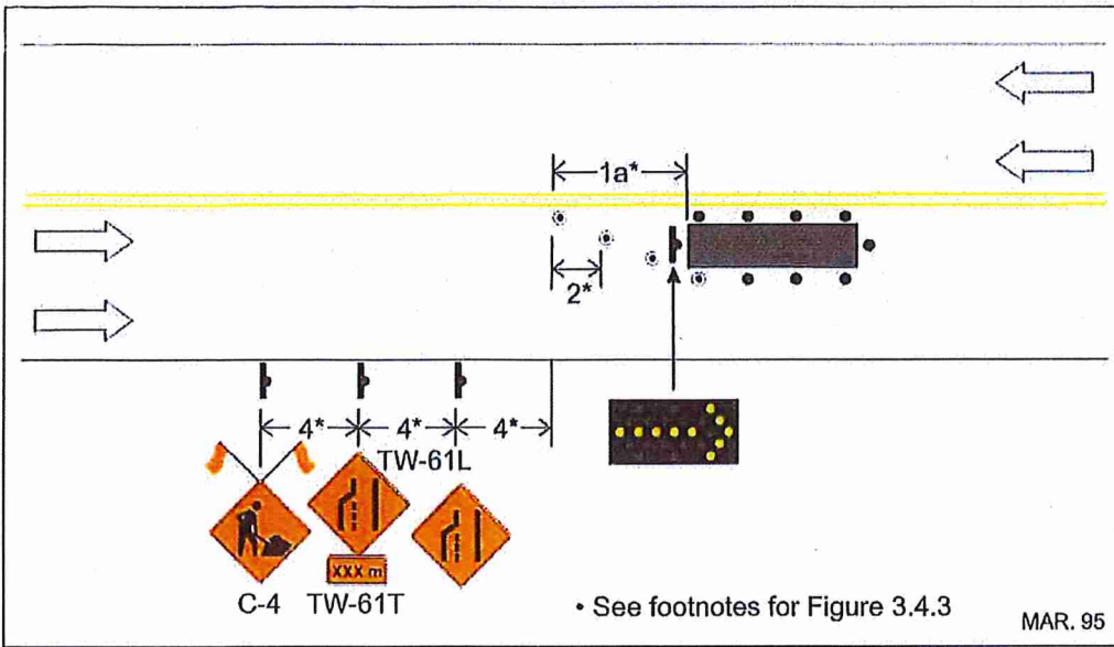
Figure 3.4.4 Left Lane Closed – Multilane Roadway
