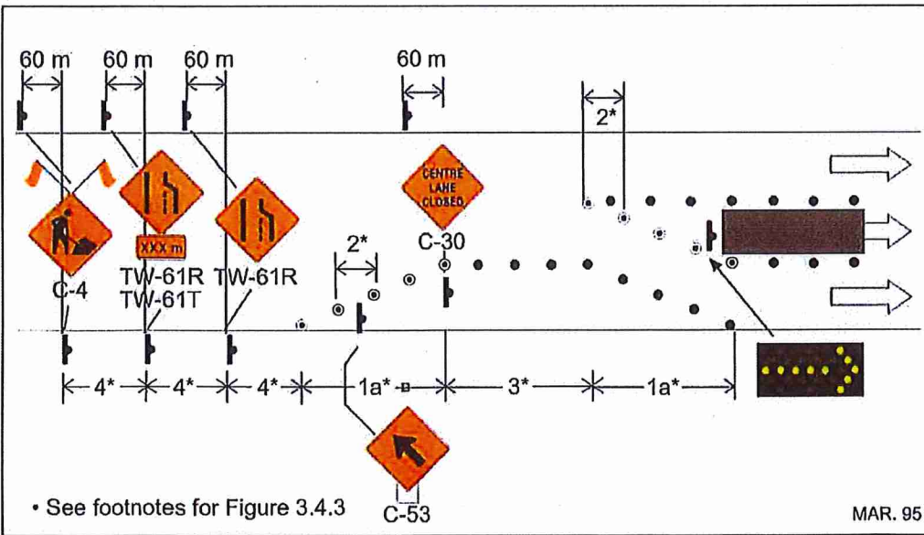
Figure 3.4.5 Centre Lane Closed – Multilane Roadway
