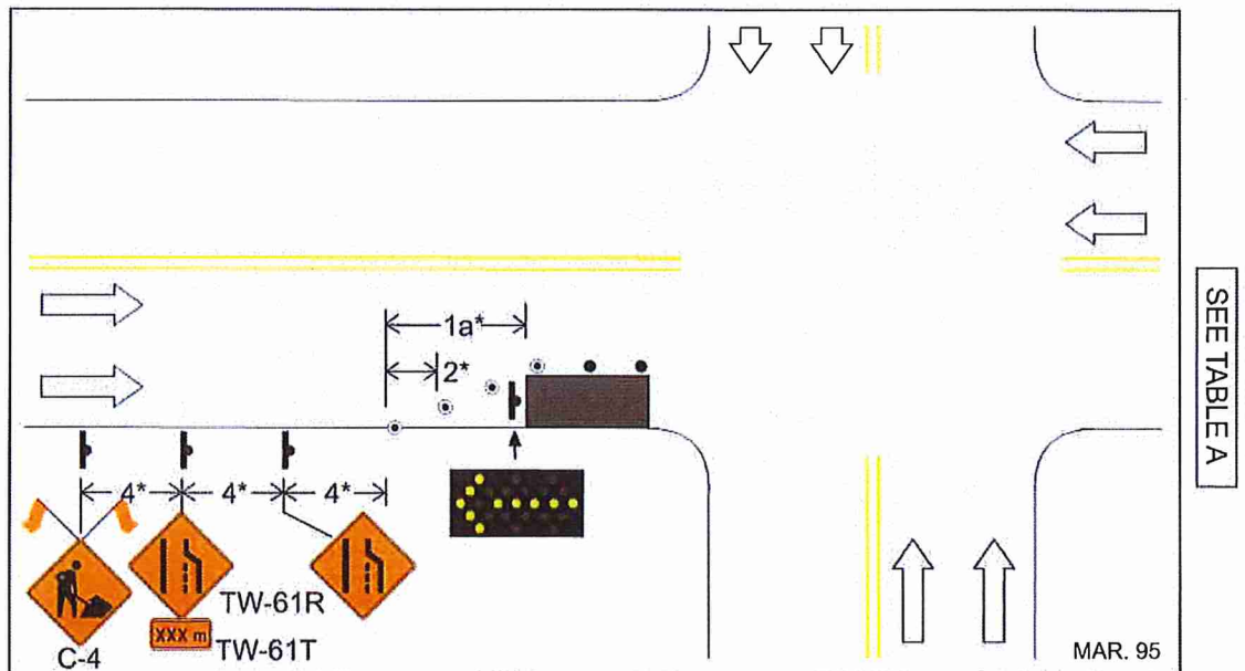
Figure 3.4.3 Right Lane Closed – Multilane Roadway
